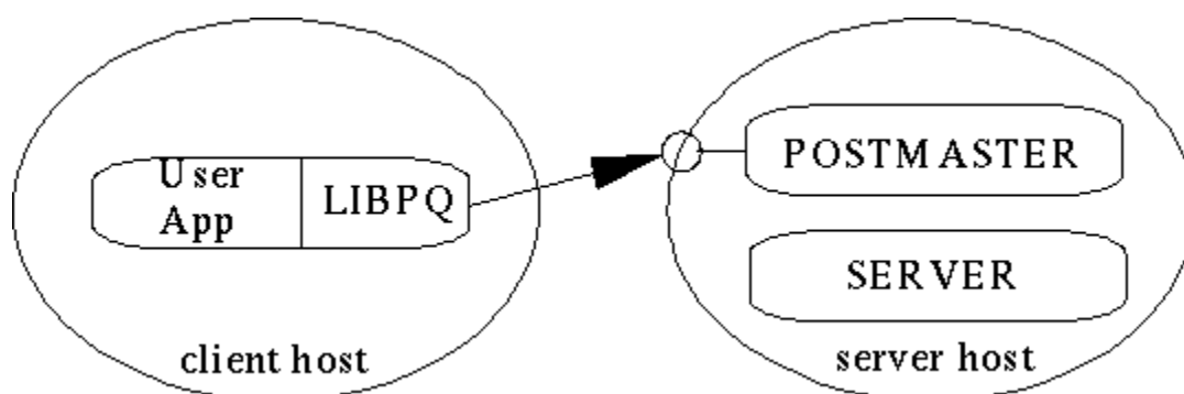
Figure 2.1. How a connection is established
