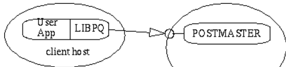
(a) frontend sends request to postmaster via well-known network socket
